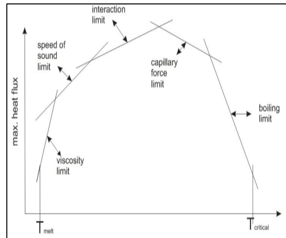
Fig. 3. Limitations of a Heat Pipe [2]
